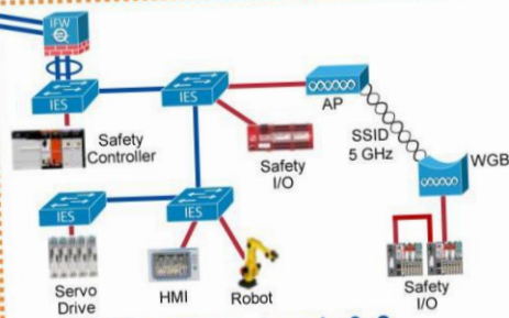
Cell/Area Zone - Levels 0–2 Linear/Bus/Star Topology
